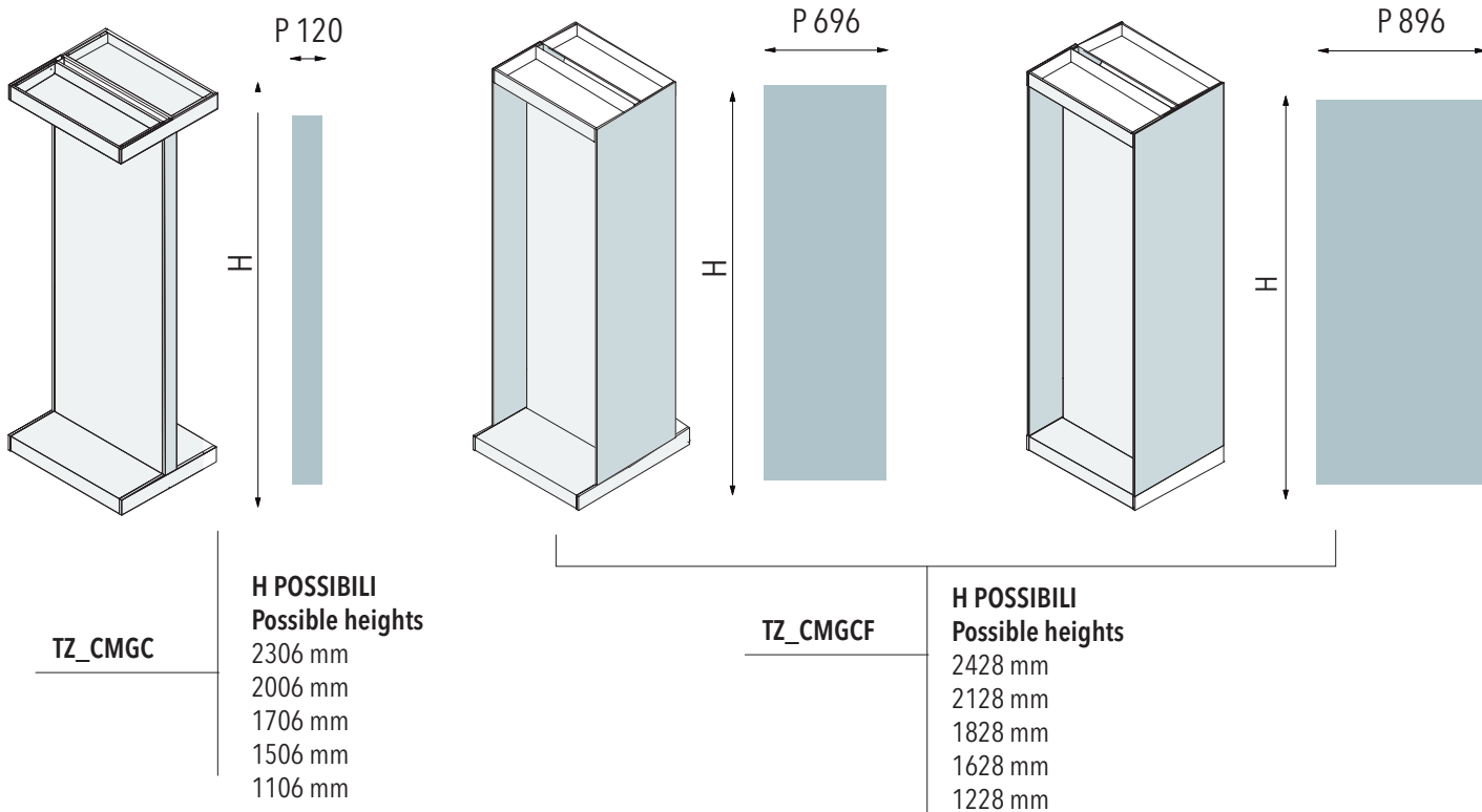
COPRIMONTANTE SI BASE SI CELINO Cover for wall upright with base and with canopy
