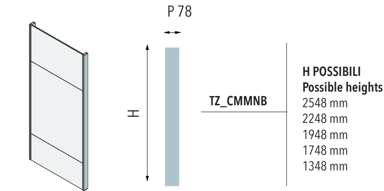
COPRIMONTANTE NO BASE NO CELINO Cover for wall upright no base no canopy
