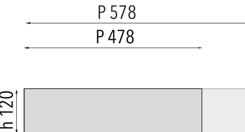
B2 COPRIBASE Cover for base
