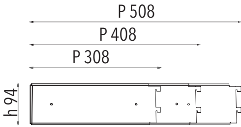
S4 STAFFA CELINO Brackets for top
