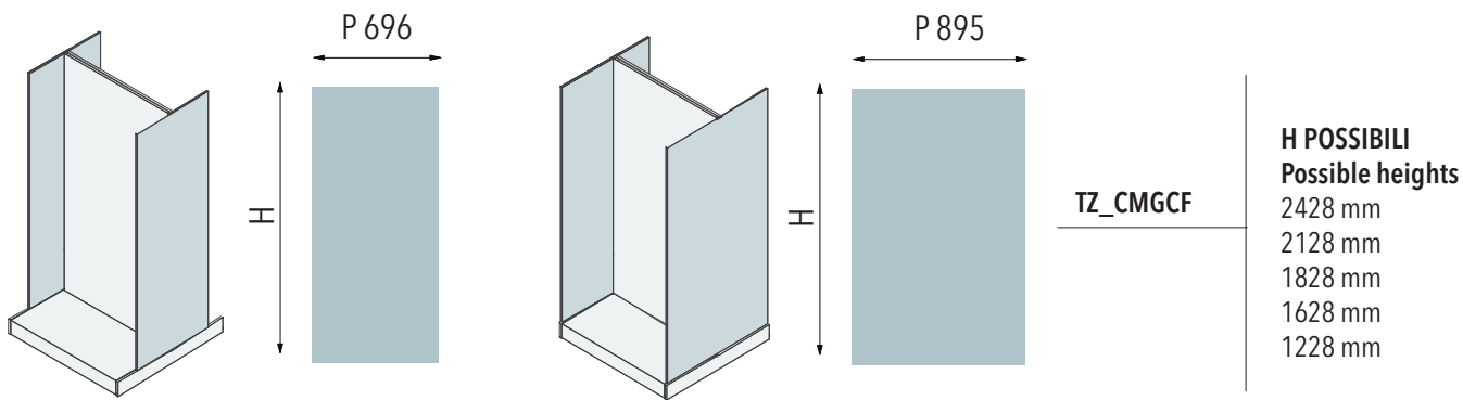
COPRIMONTANTE SI BASE SI CELINO Cover for wall upright with base and with canopy
