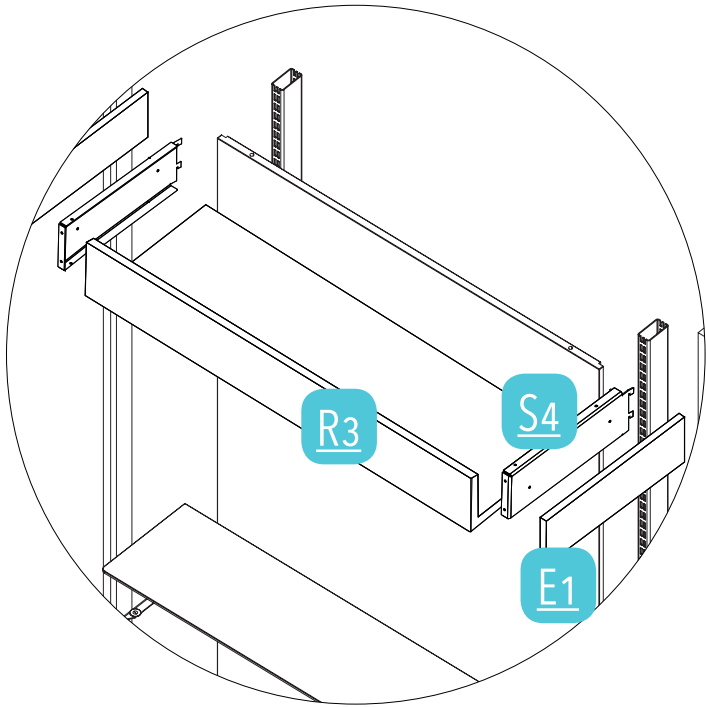
S4 STAFFA CELINO Brackets for top
