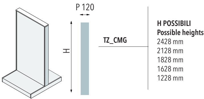
COPRIMONTANTE SI BASE NO CELINO Cover for upright with base no canopy
